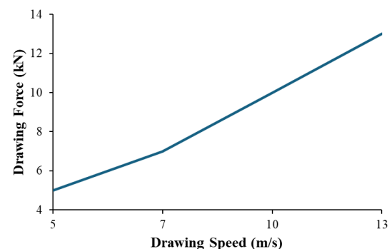
Fig.10. Comparison of FEM-based drawing force results
