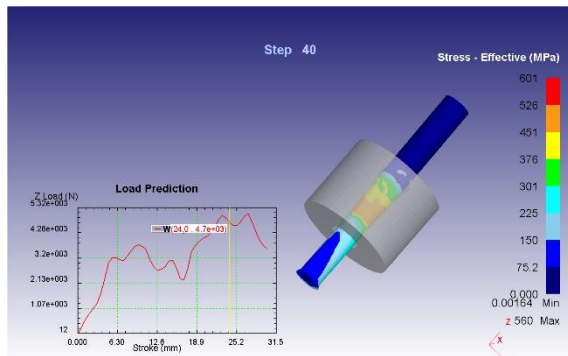
Fig. 3. Effective stress distribution at 7 m/s.
