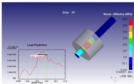
Fig. 5. Effective stress distribution at 13 m/s.
