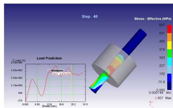
Fig. 2. Effective stress distribution at 5 m/s.
