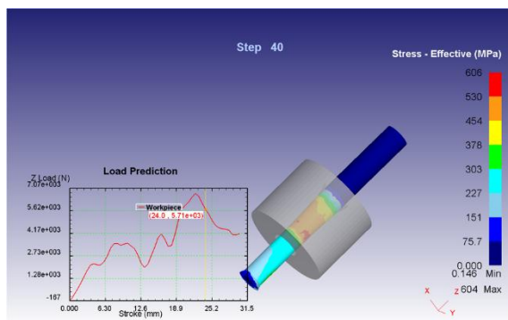
Fig. 4. Effective stress distribution at 10 m/s.
