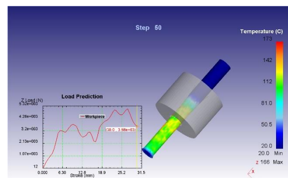
Fig. 7. Temperature distribution at 7 m/s.
