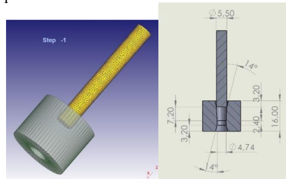
Fig. 1. A-)FEM model and b-) dimensions of the wire drawing process.
