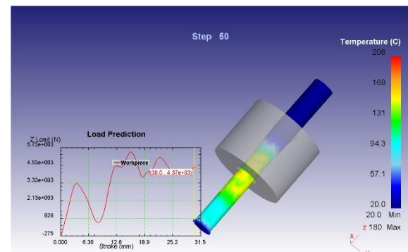
Fig. 6. Temperature distribution at 5 m/s.
