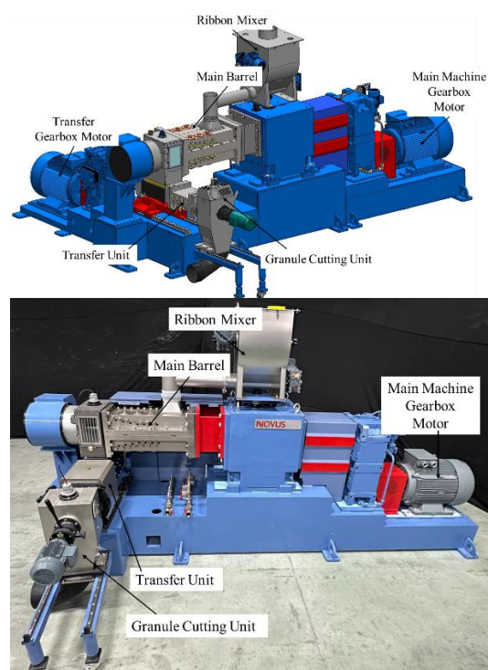
Fig. 4. Compound production machine parts
