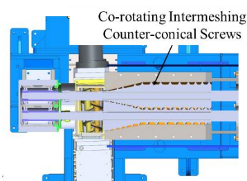
Fig. 5. Co-rotating Intermeshing Counter-conical Screws
