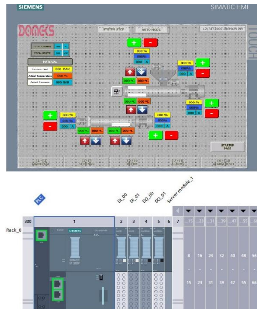
Fig. 3. Main Control Panel and PLC unit
