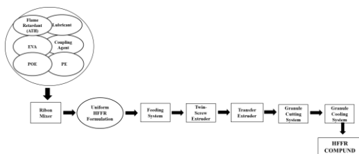
Fig. 1. HFFR Compound Production Chart
