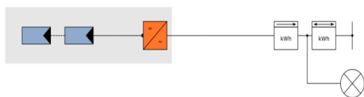
Fig. 1. Schematic Diagram of the Grid-Connected Photovoltaic (PV) System [16].
