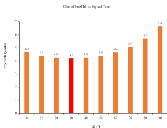
Fig. 3. Variation of Payback Period with Tilt Angle for the PV System in Edirne, Türkiye [16].
