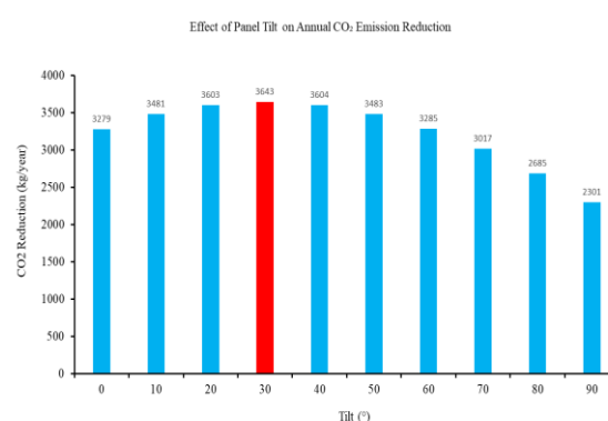
Fig. 4. Variation of CO 2 Reduction with Tilt Angle for the PV System in Edirne, Türkiye [16].
