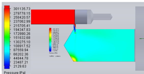
Fig. 5. Pressure distribution in the cavitator
