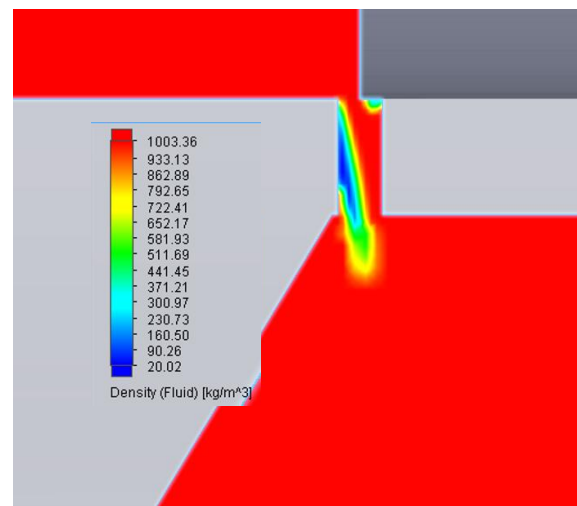
Fig. 8. Fluid density distribution in the throttling gap
