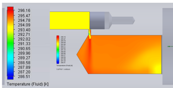
Fig. 6. Fluid temperature distribution in the cavitator
